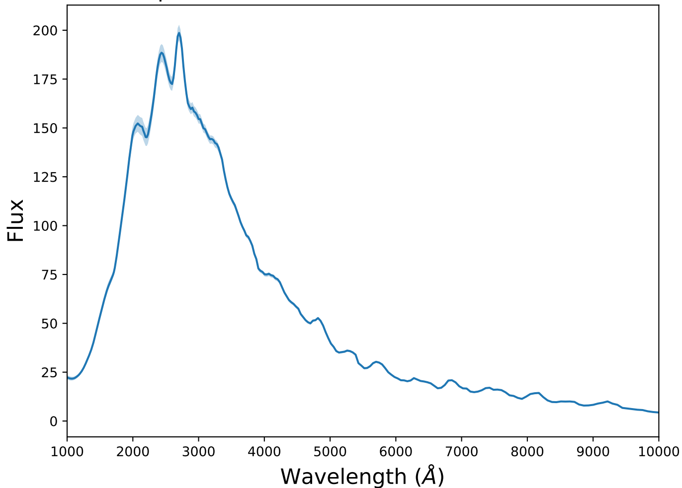
Spectrum 1 for transient CCSN at z=0.61
